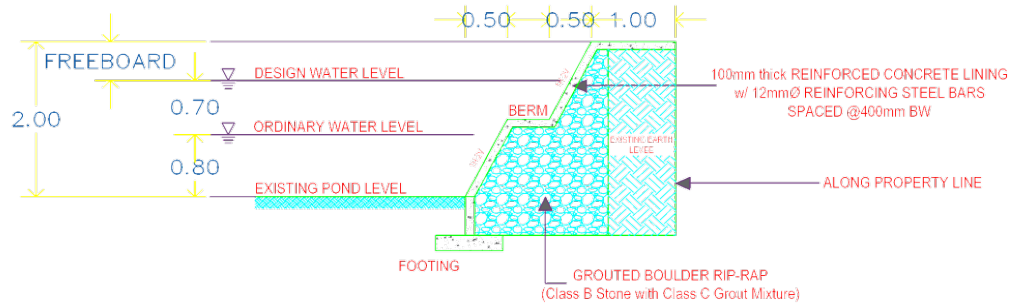
TRANSVERSE SECTION FOR DIKE C
