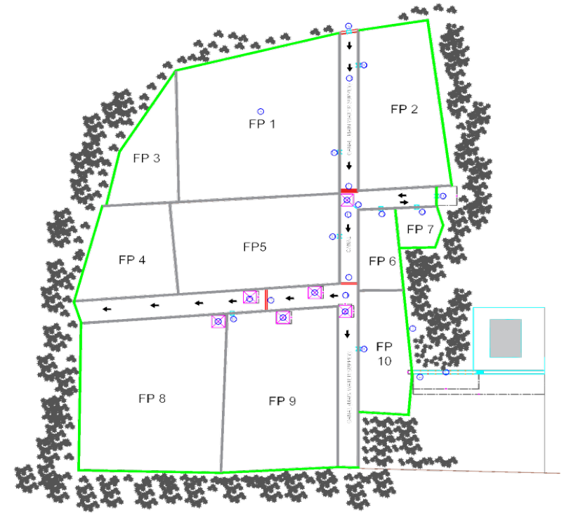
DIKE "C" AREA OF COVERAGE
