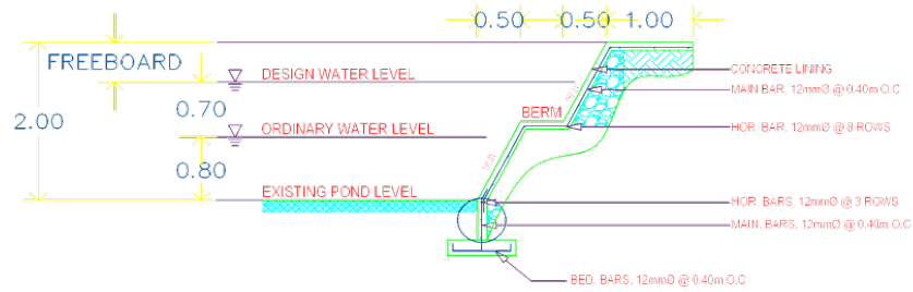
REINFORCEMENT DETAIL FOR DIKE C
