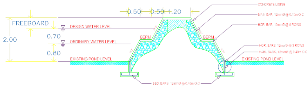
REINFORCEMENT DETAIL FOR DIKE B
