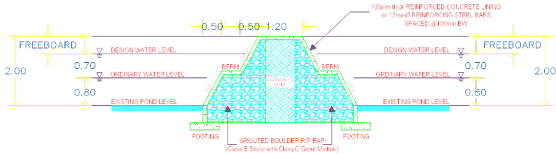
TRANSVERSE SECTION FOR DIKE B
