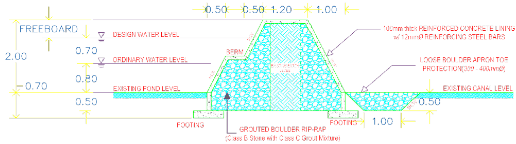
TRANSVERSE SECTION FOR DIKE A
