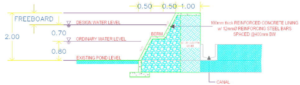
CANAL SECTION ALONG DIKE C
