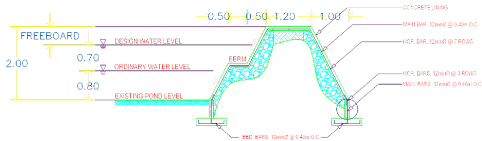
REINFORCEMENT DETAIL FOR DIKE A
